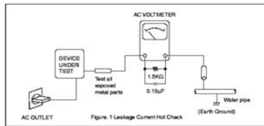
Figure 1 Leakage Current Hot Check
